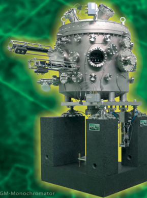
REIXS VLS-PGM-Monochromator CLS
