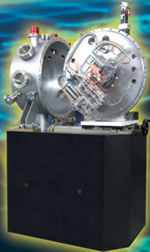
Liquid nitrogen-cooled DCM DLS
