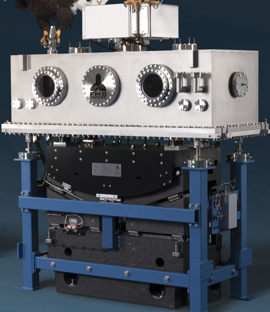
HIGH HEAT LOAD MIRROR SYSTEMS | 19-ID BEAMLIN @ APS | USA
